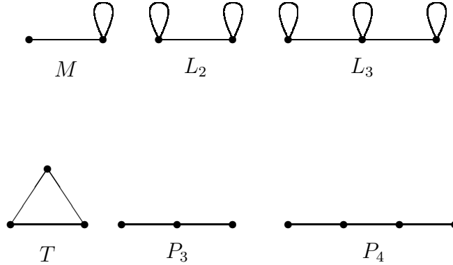
FIGURE 1. Forbidden Subgraphs
