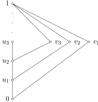
FIGURE 2. \text{Con}(\mathbf{S}, +, 0) does not satisfy the infinite analogue of Theorem 22.
