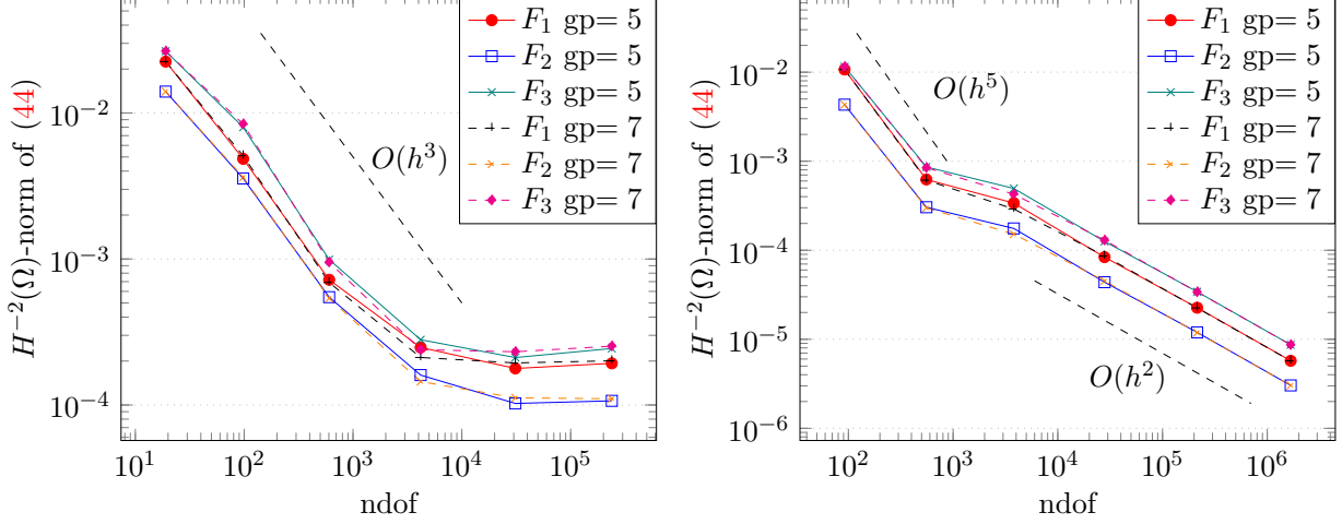
Figure 2: Convergence of the three functionals in (44) in the H^{-2}(\Omega) -norm with respect to number of degrees of freedom (ndof) for 5 and 7 Gauss points (gp) in dimension N = 3 . Left: r = 0 . Right: r = 1 .
